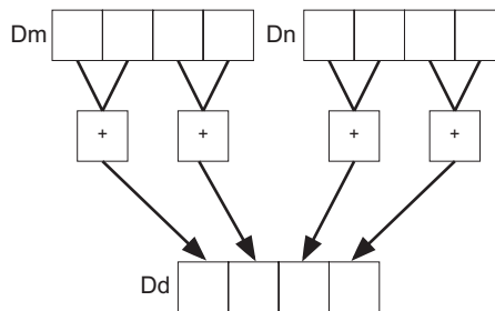
Figure A8-3 Operation of VPADD for data type I16
