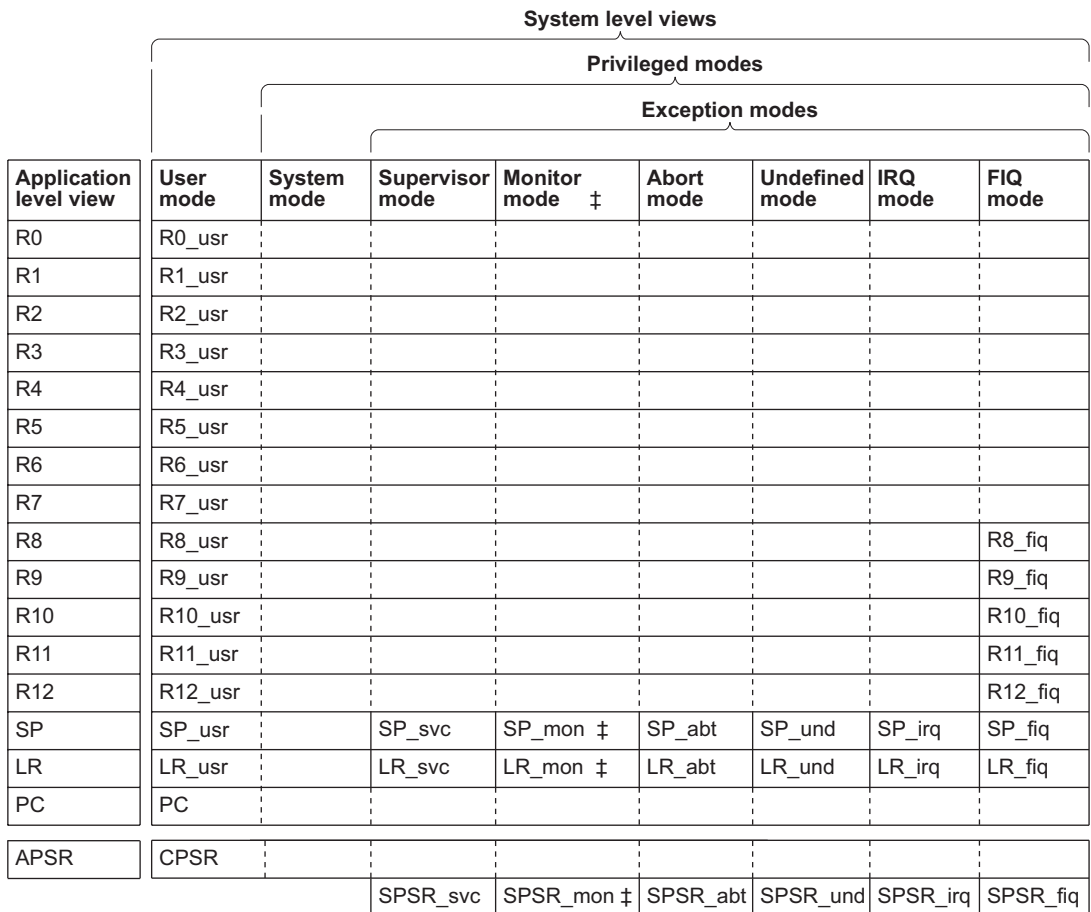
Figure B1-1 Organization of general-purpose registers and Program Status Registers
