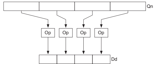
Figure A4-4 Advanced SIMD instruction producing narrower result
