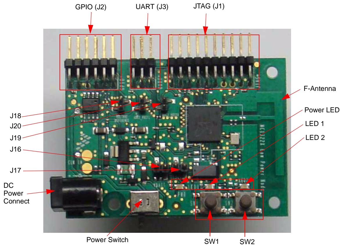
Figure 3-4. 1322x-LPN PCB Top View
