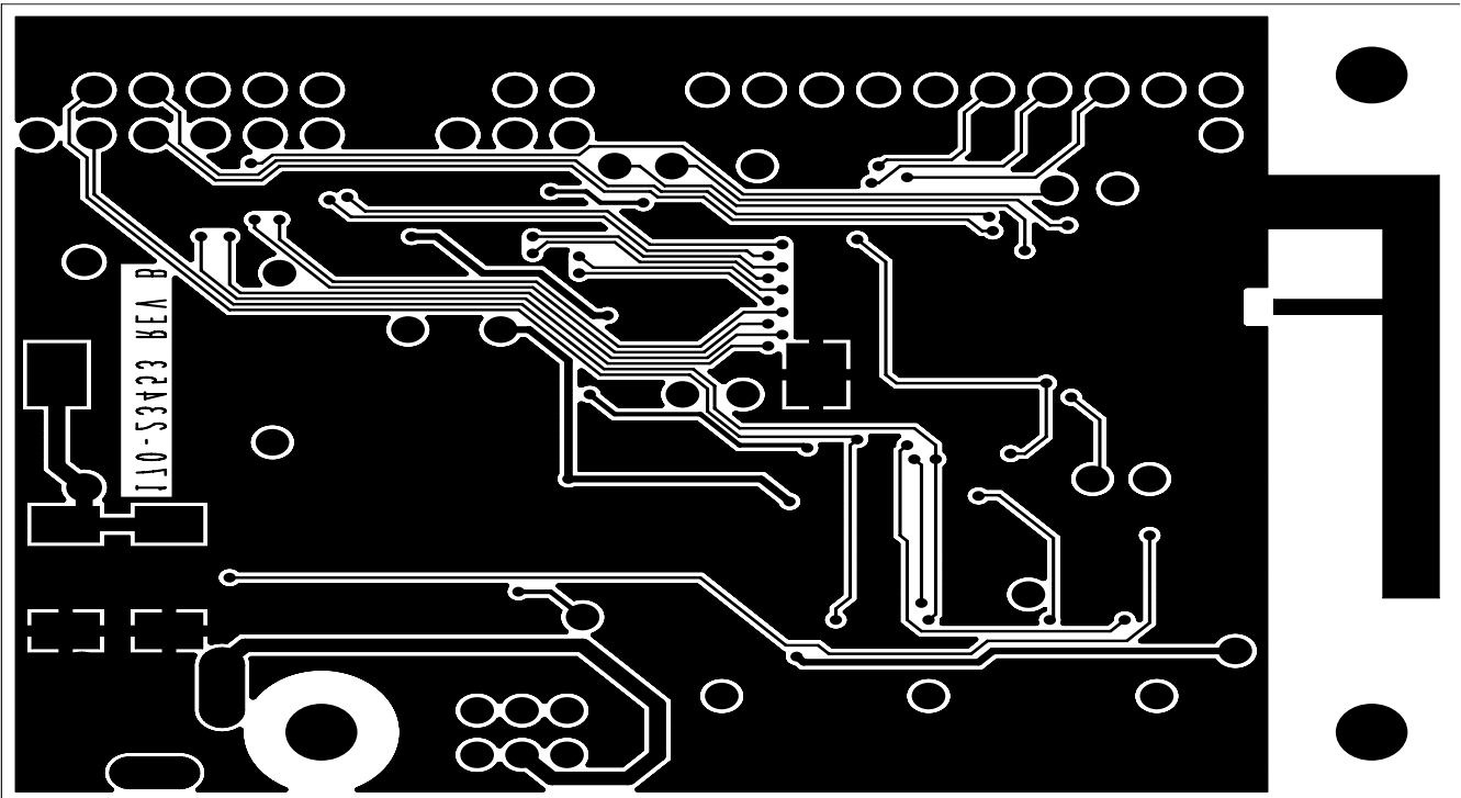
Figure 4-5. 1322x-LPN PCB Layout (Bottom View)
