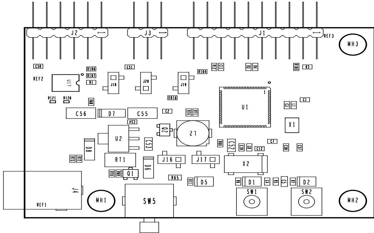
Figure 4-2. 1322x-LPN PCB Component Location (Top View)
