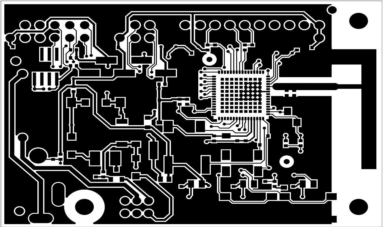
Figure 4-4. 1322x-LPN PCB Layout (Top View)
