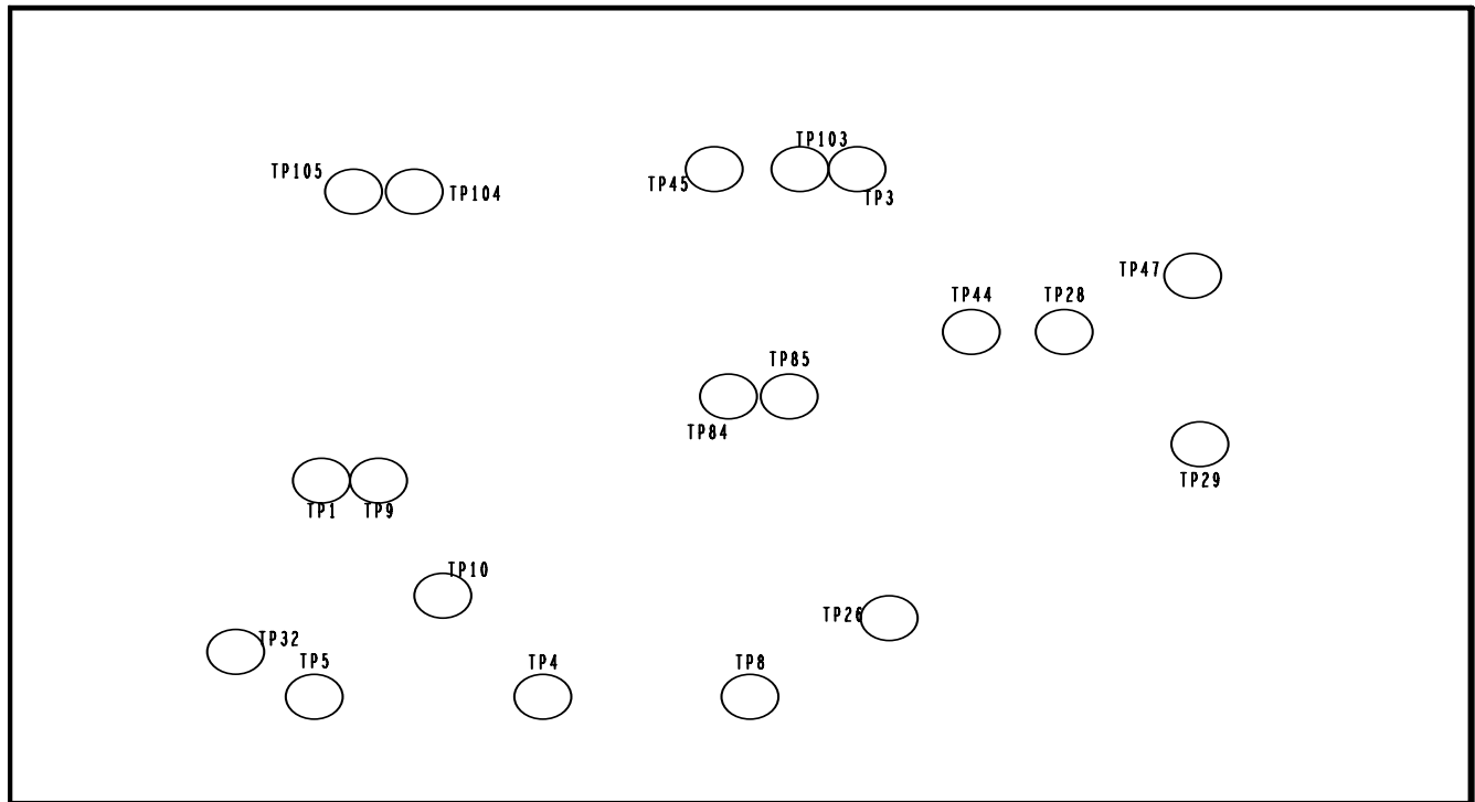
Figure 4-3. 1322x-LPN PCB Test Points (Bottom View)
