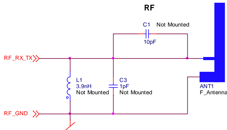
Figure 3-5. 1322x-LPN RF Network.
